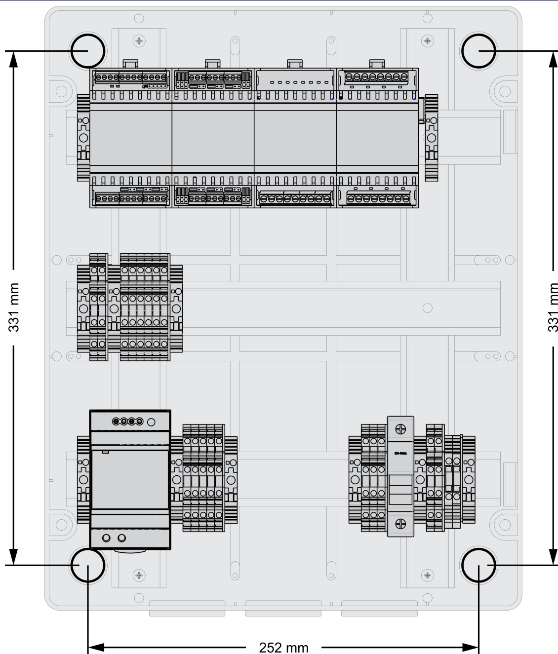
Figure 8: Mounting holes position
