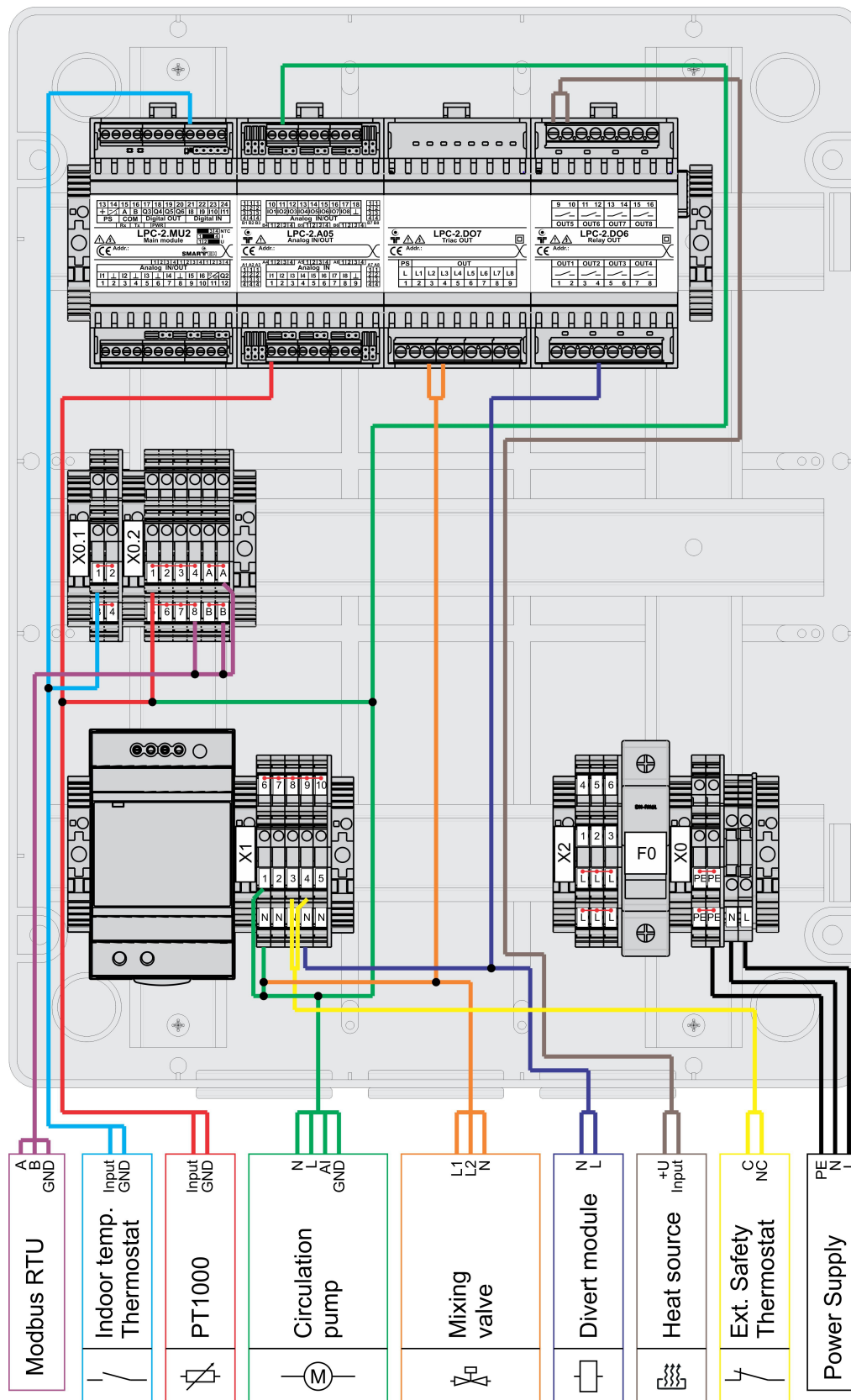
Figure 2: SHC-001 schematic example of device connections
