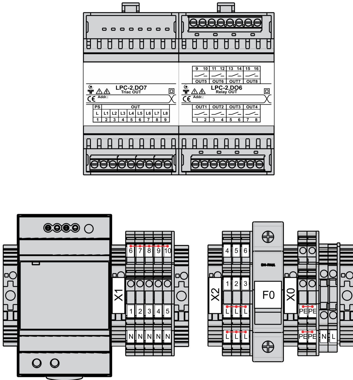
Figure 6: SHC-001 inside, power section
