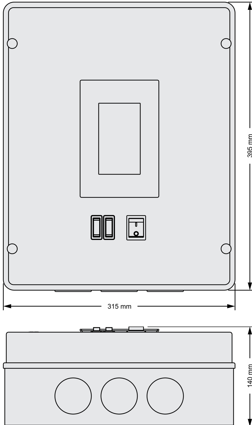
Figure 7: Housing dimensions
