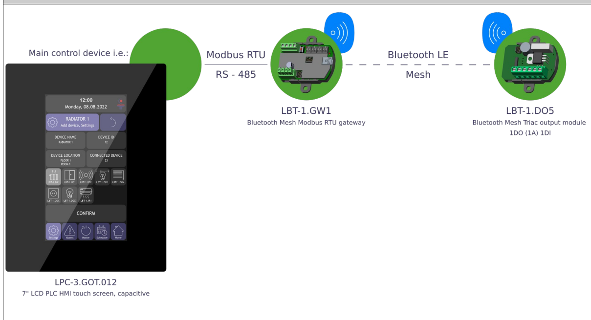
Figure 2: LBT-1.DO5 device connection
