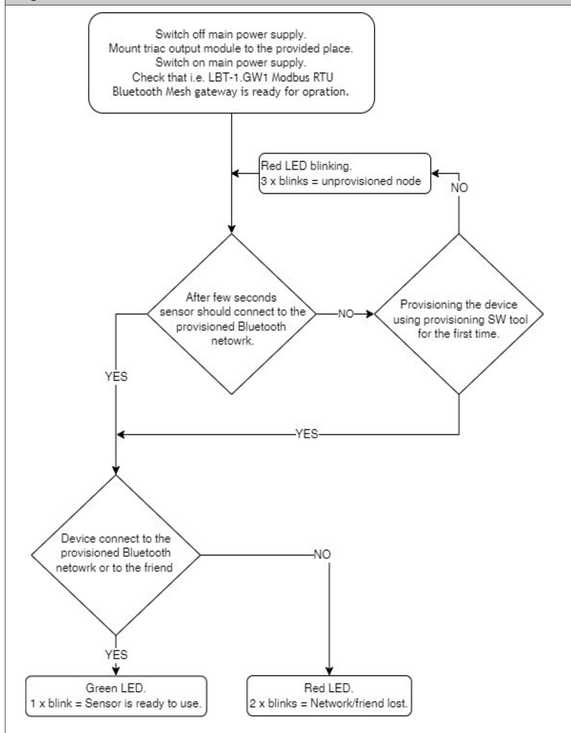
Figure 8: Installation flowchart
