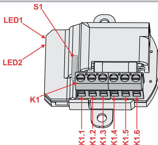
Figure 5: LBT-1.D05 module
