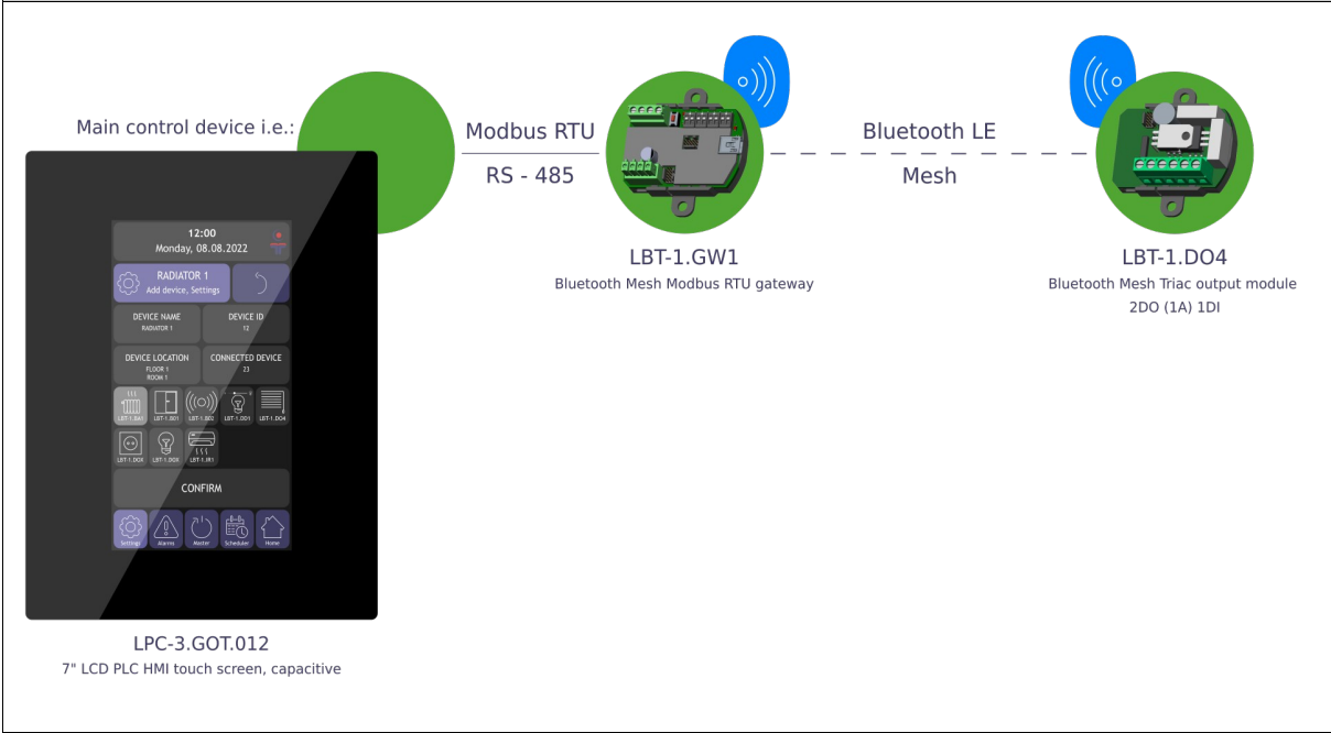
Figure 2: LBT-1.DO4 device connection
