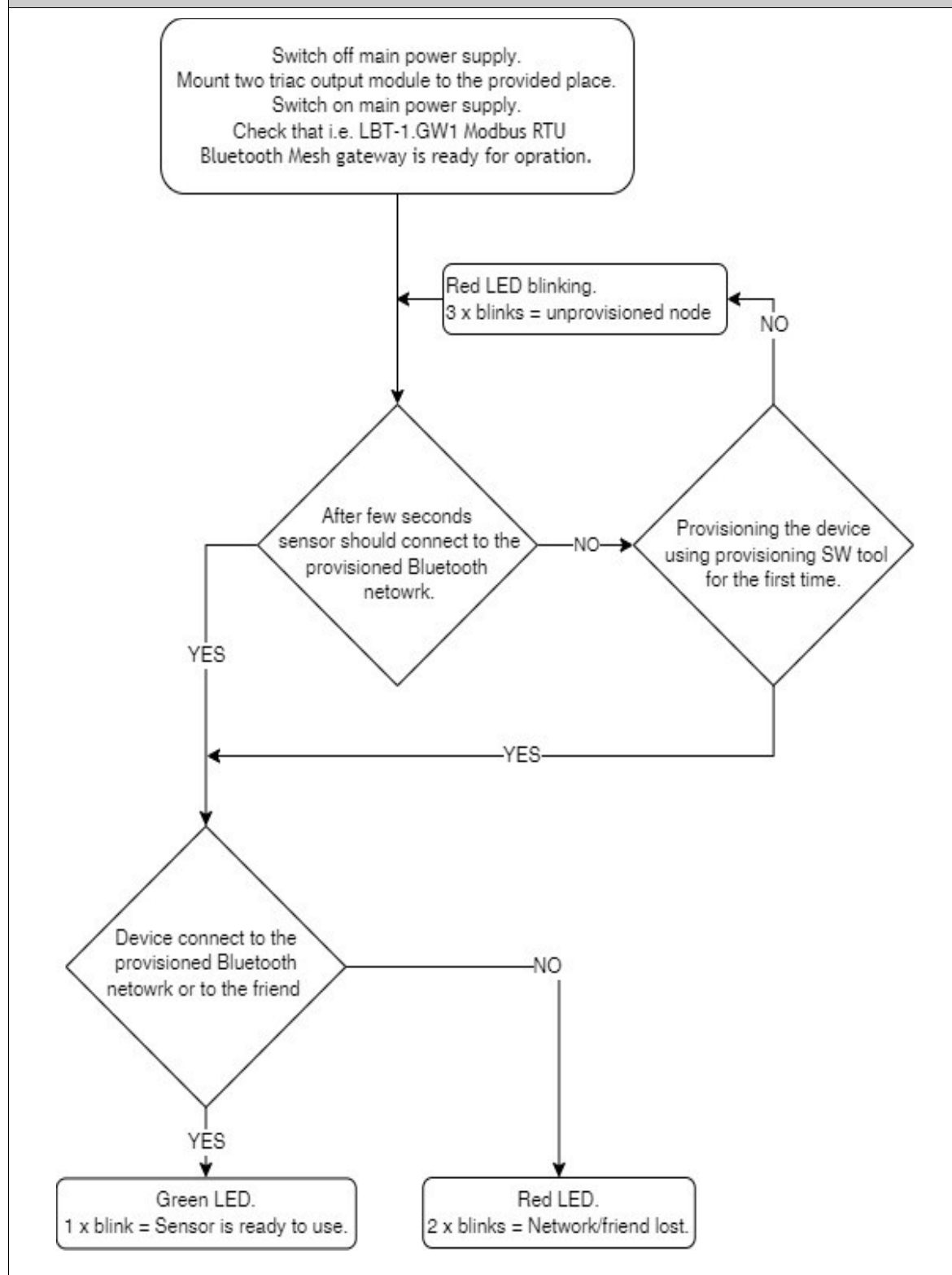
Figure 8: Installation flowchart
