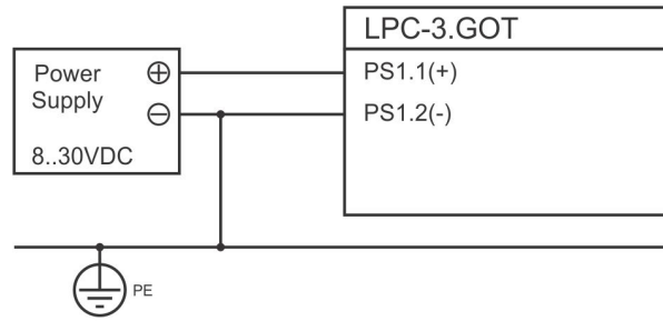
Figure 7: Grounding possibilities
