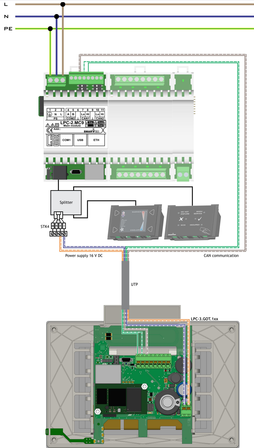
Figure 6: Example of power supply from main module and CAN communication
