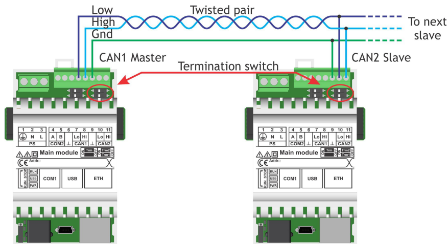
Figure 8: CAN Master and Slave wiring diagram example
