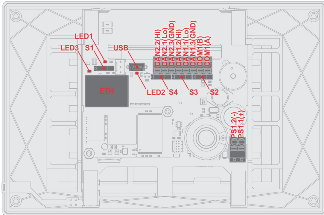
Figure 3: Connection scheme
