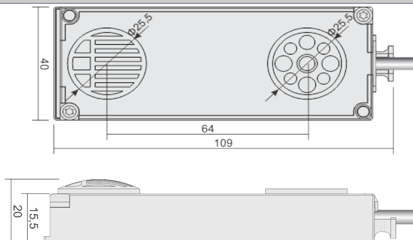
Figure 3: Housing dimensions
