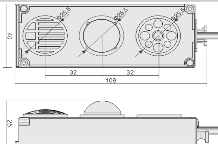
Figure 3: Housing dimensions
