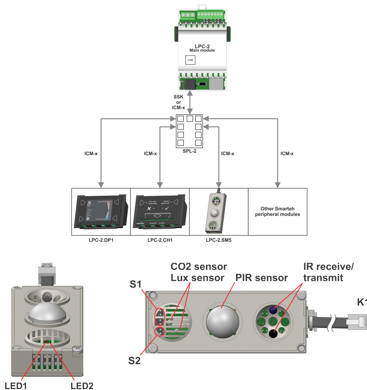
Figure 2: Connection scheme
