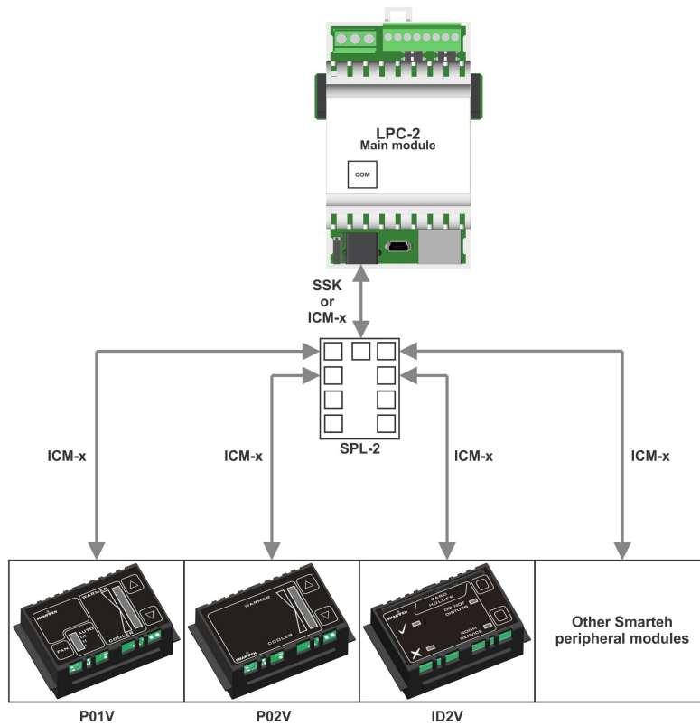
Figure 2: Connection scheme
