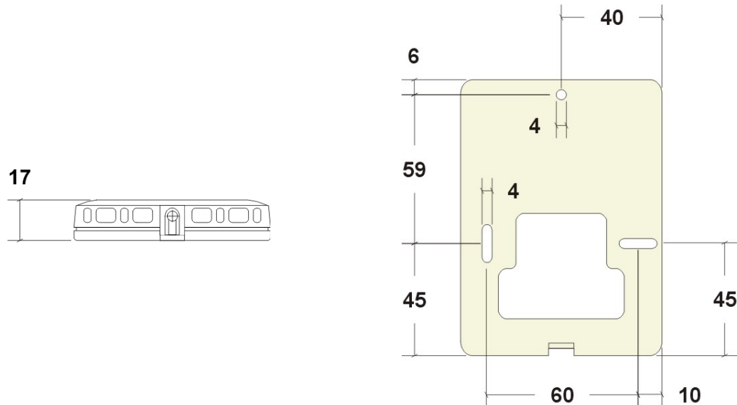
Figure 3: Housing dimensions
