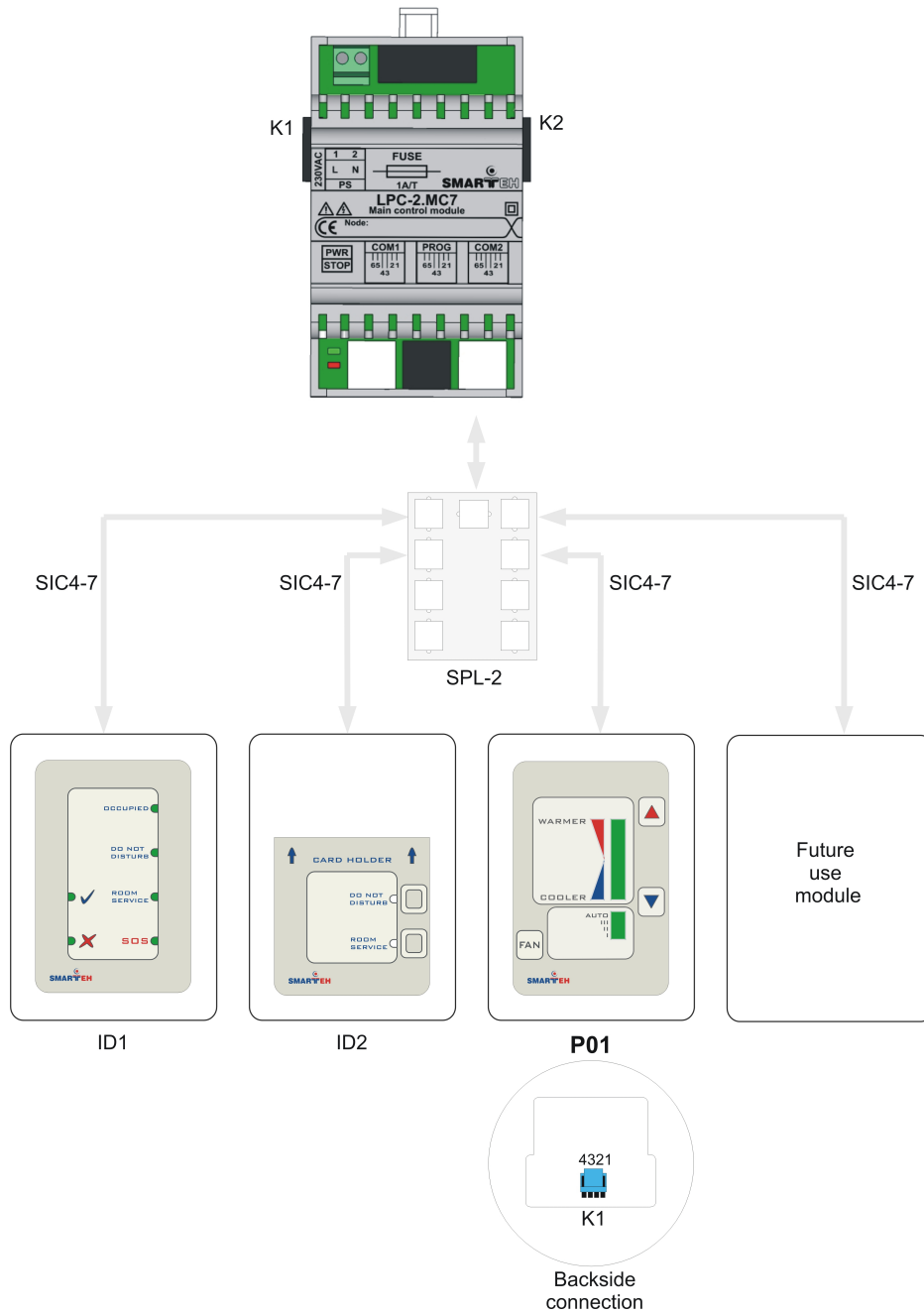
Figure 2: Connection scheme
