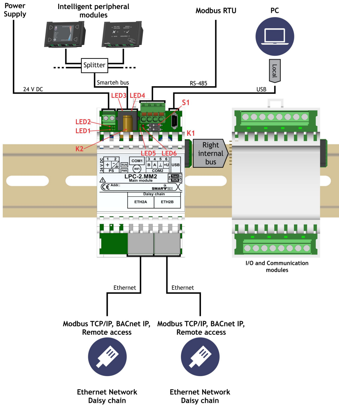
Figure 2: Connection scheme
