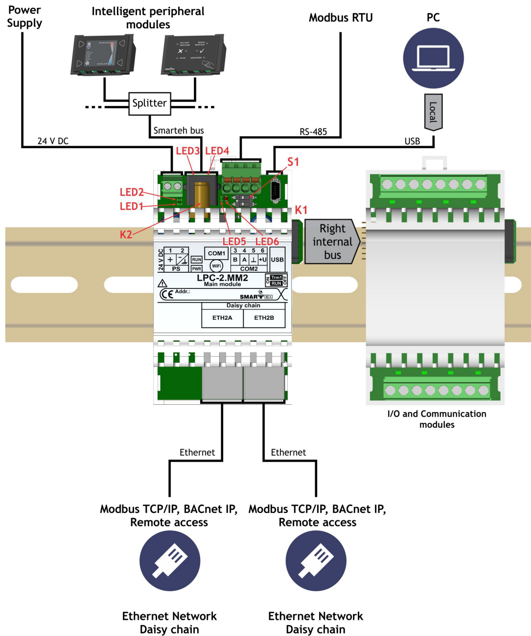
Figure 2: Connection scheme
