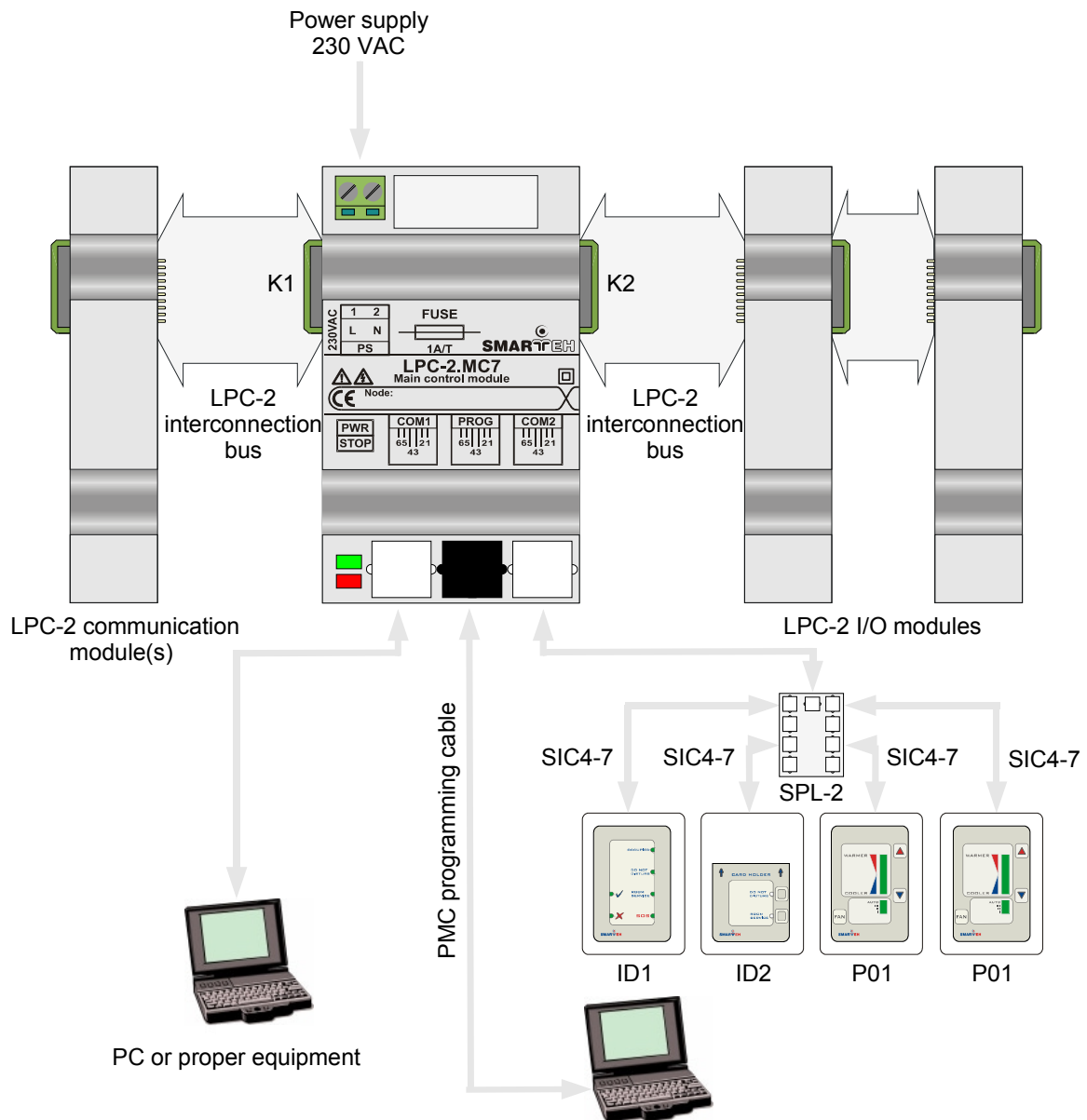
Figure 2: Connection scheme
