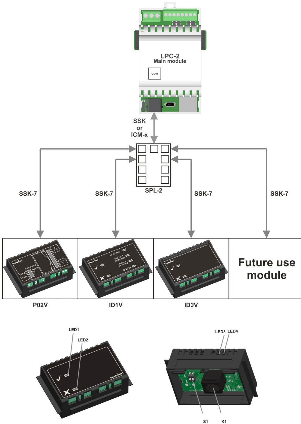
Figure 2: Connection scheme
