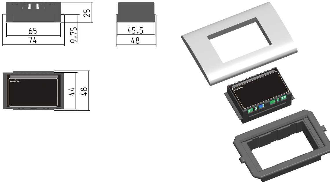
Figure 4: Housing dimensions
