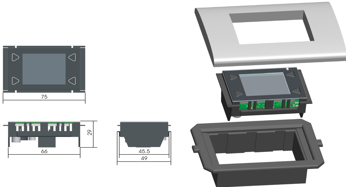
Figure 3: Housing dimensions
