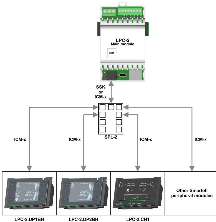
Figure 2: Connection scheme
