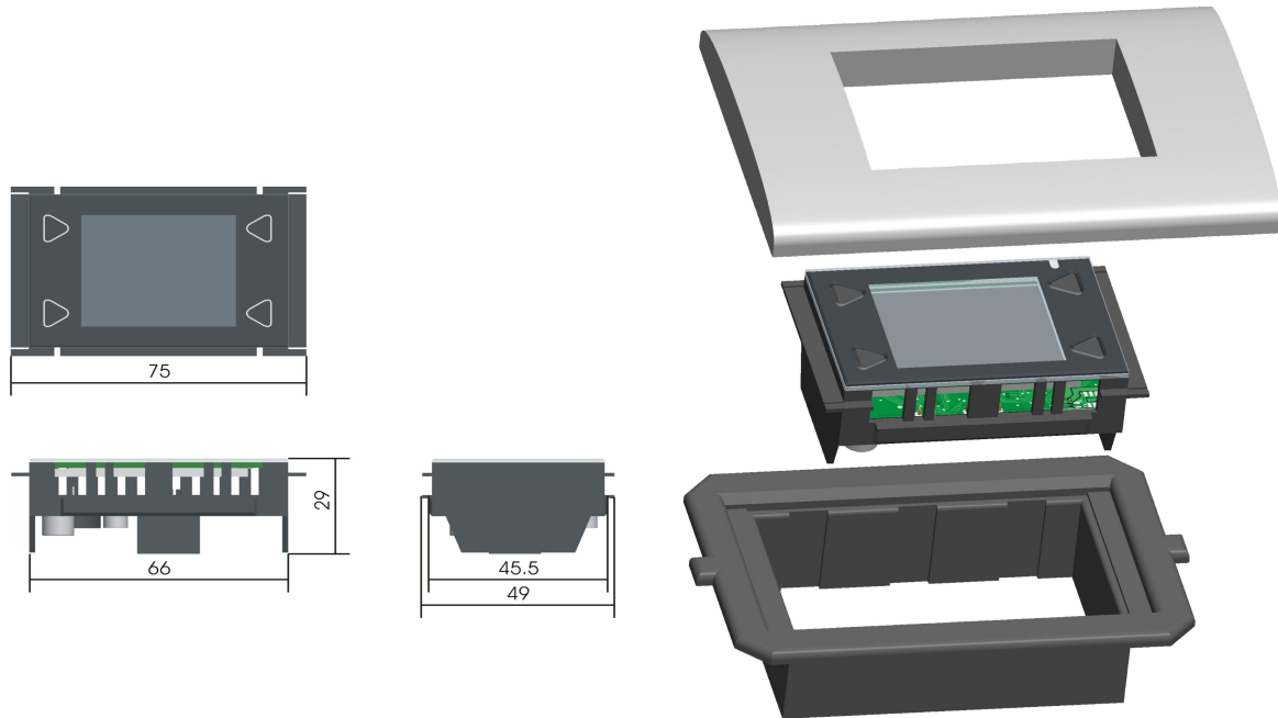
Figure 3: Housing dimensions
