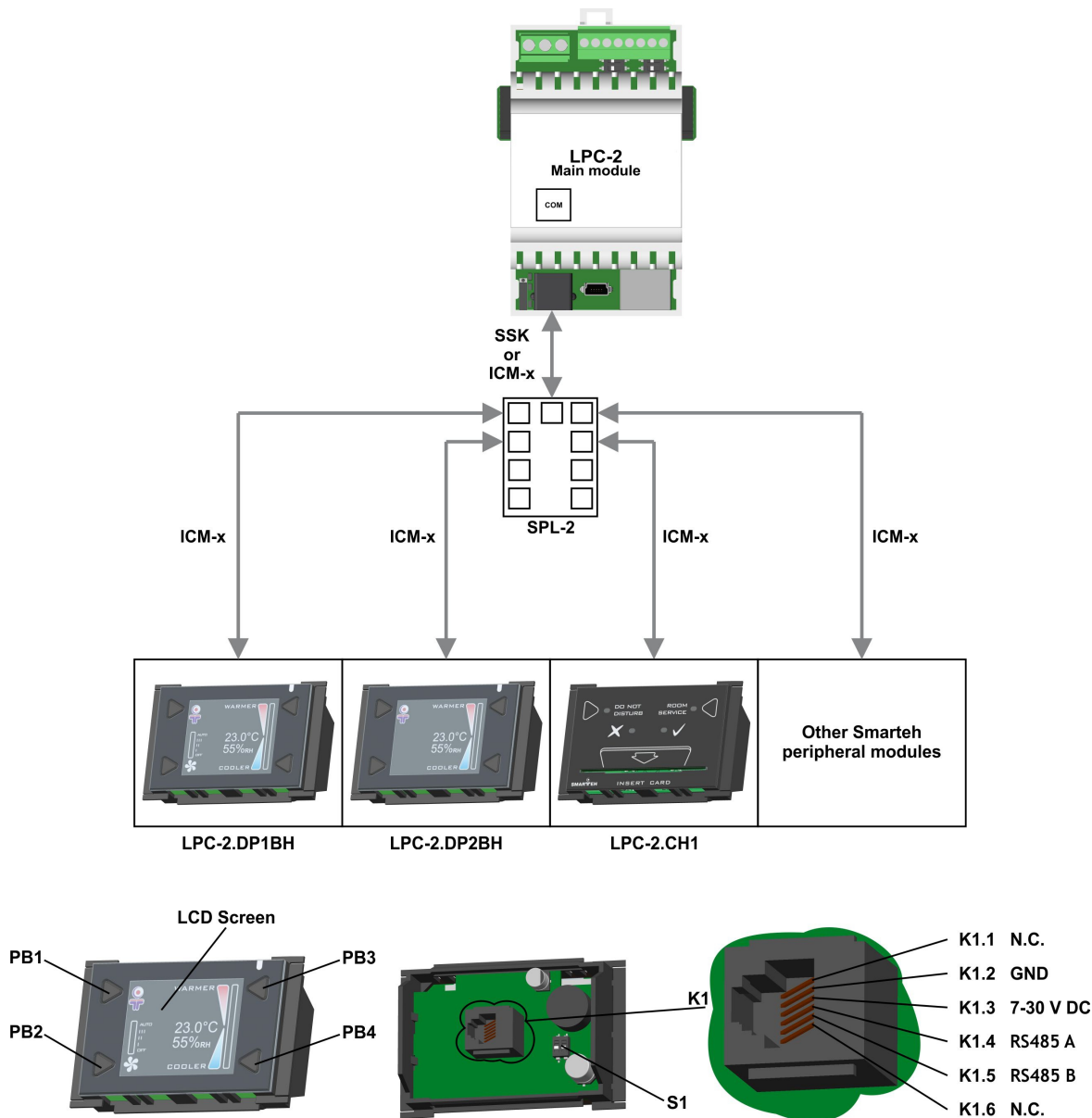
Figure 2: Connection scheme
