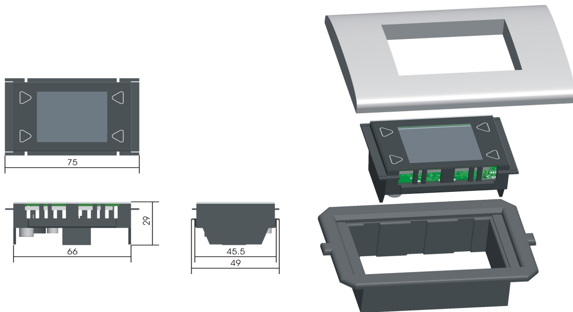
Figure 3: Housing dimensions
