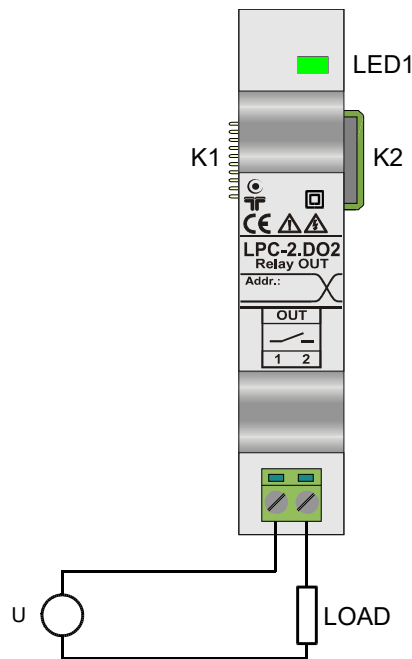
Figure 2: Connection scheme
