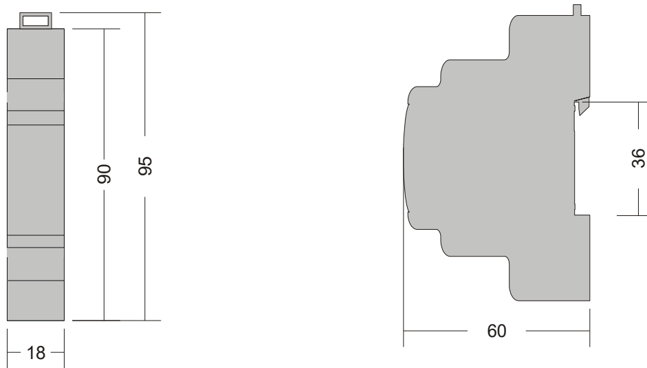
Figure 3: Housing dimensions
