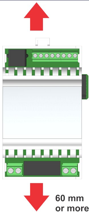
Figure 5: Minimum clearances
