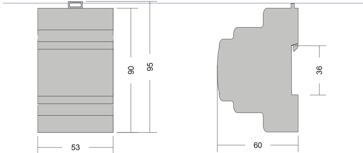
Figure 3: Housing dimensions
