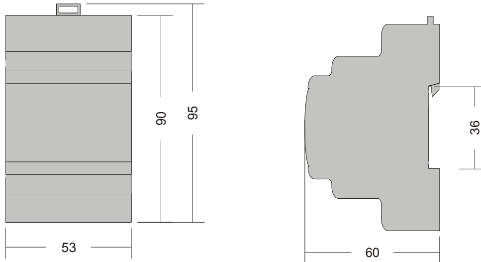
Figure 3: Housing dimensions
