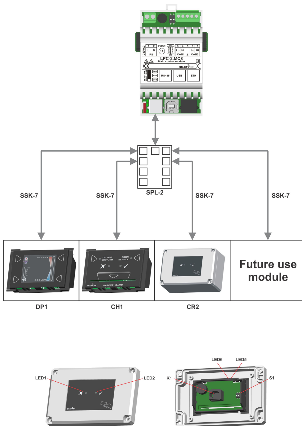
Figure 2: Connection scheme
