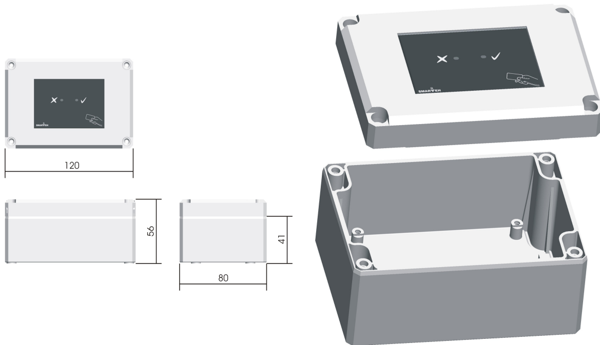
Figure 3: Housing dimensions
