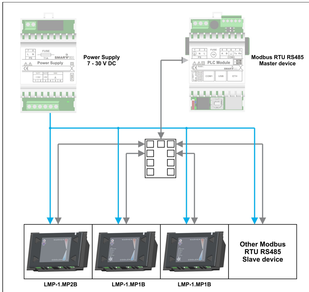
Figure 2: Connection scheme
