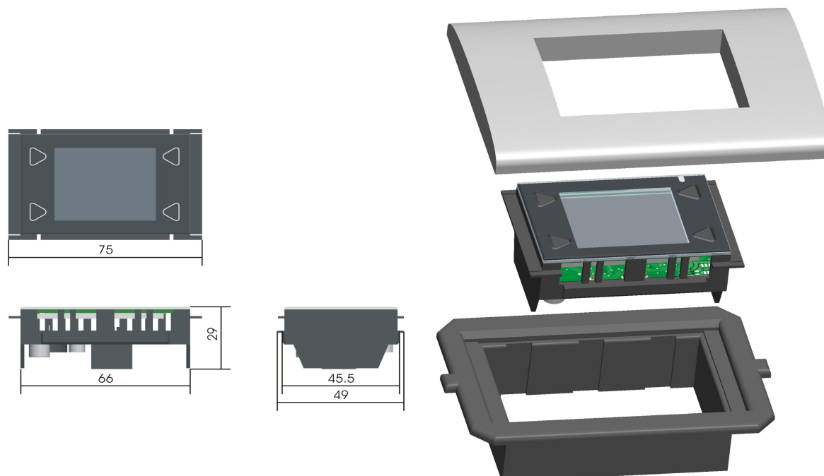
Figure 3: Housing dimensions
