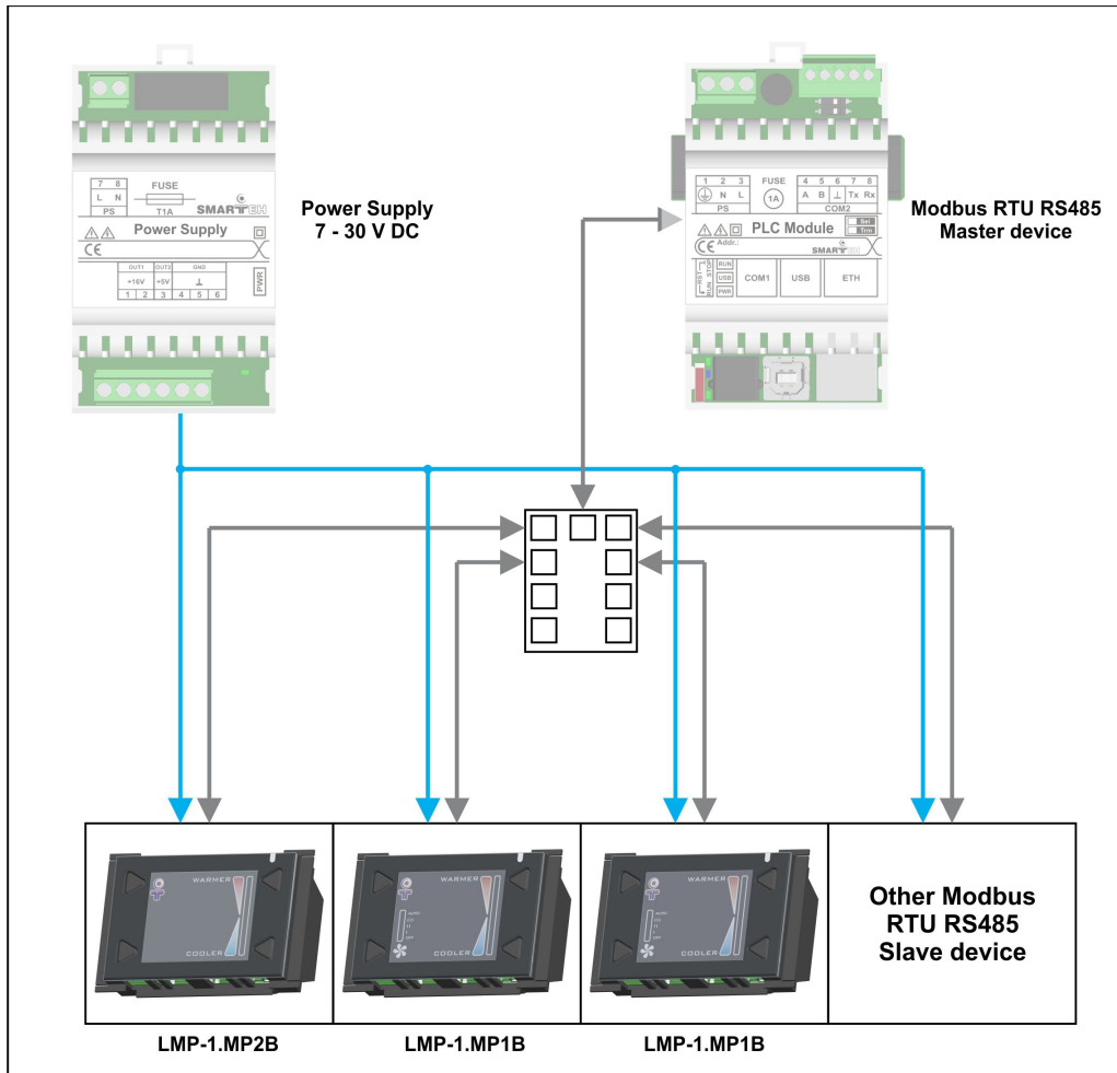
Figure 2: Connection scheme
